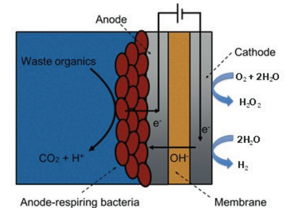
Figure 2: Schematic of an MxC to produce H 2 or H 2 O 2 from organics in dairy wastewater.
