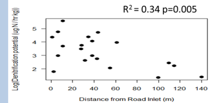
Figure 2: Graph of Distance from Road Inlet (m) and Log (Denitrification Potential (ug N/hr kg))
