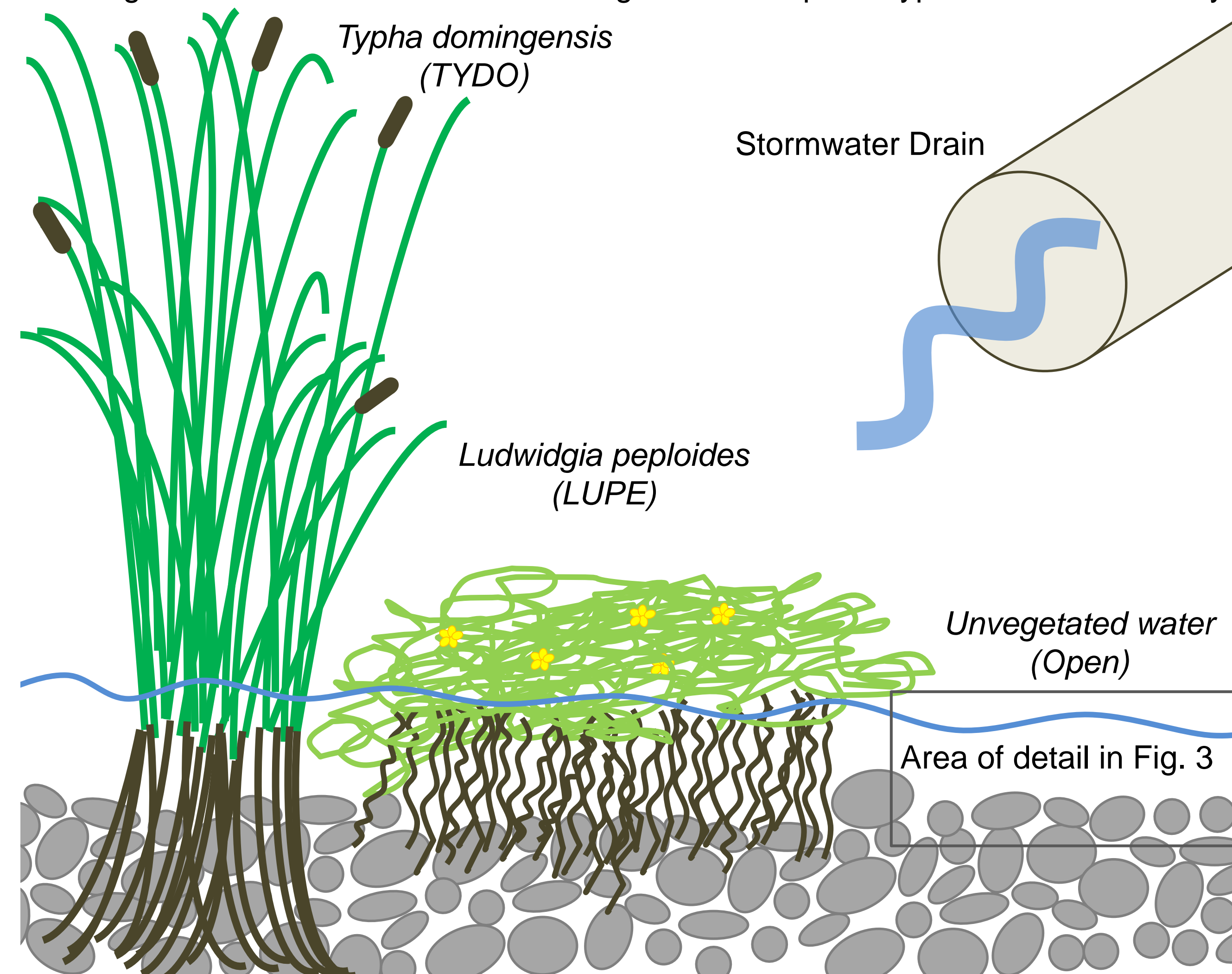
Figure 1. Schematic of wetland configuration and patch types used in this study.
