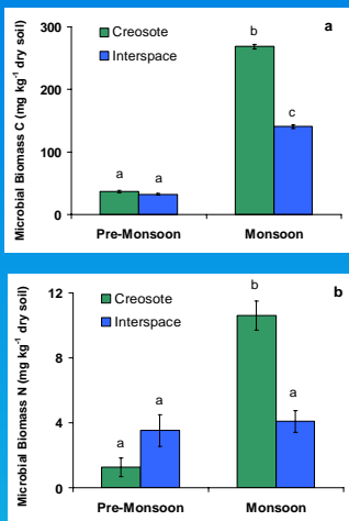
Figure 1: Microbial biomass (a) C and (b) N by cover type and season. Error bars represent SEM +/- 1 SE. Letters above bars indicate significant differences using Tukey's HSD, \alpha = 0.05 . rmANOVA C: time x treatment: F=9.15_{1,20} , p=0.007 ; rmANOVA N: time x treatment: F=7.45_{1,20} , p=0.013 .
