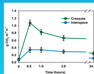
Figure 4: Average CO 2 flux rates by cover type following artificial precipitation event. Error bars represent SEM +/- 1 SE.
