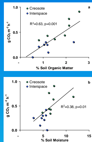
Figure 3: Soil respiration as a function of soil organic matter (a) and soil moisture (b).
