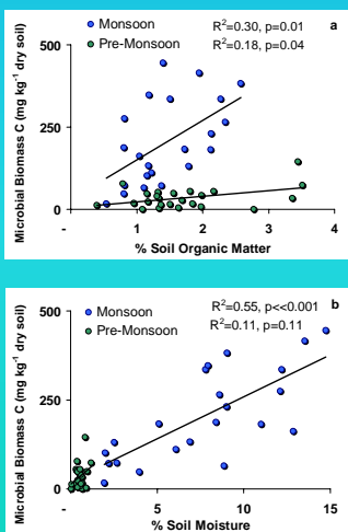
Figure 2: Microbial biomass C as a function of (a) soil organic matter and (b) soil moisture.
