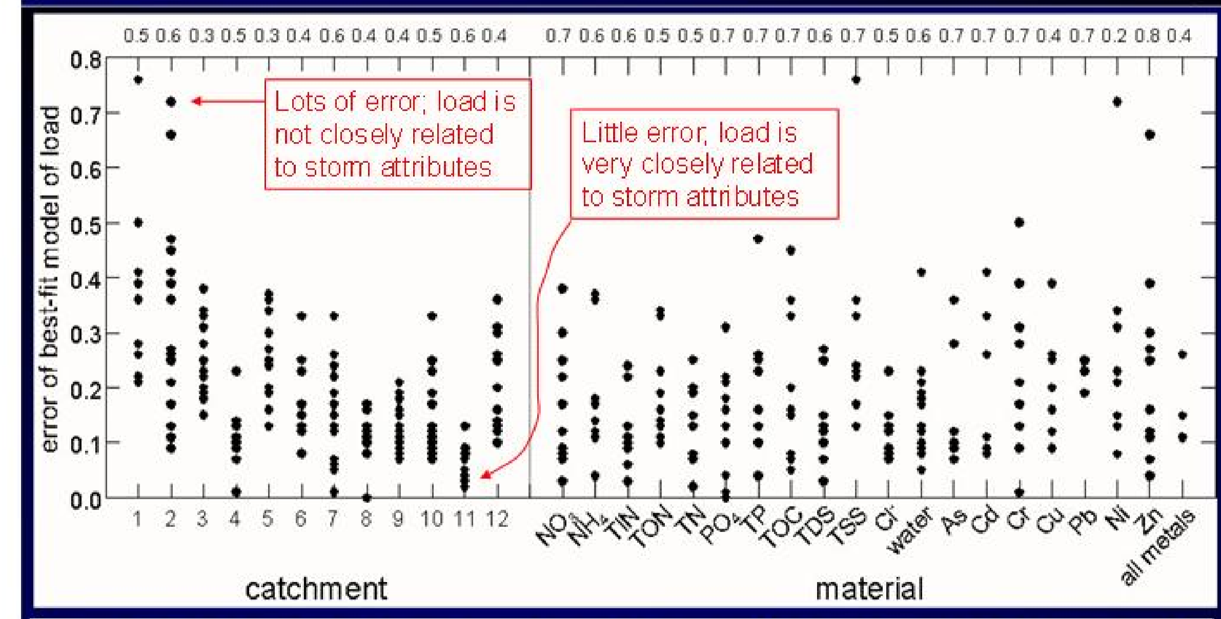
Figure 7. Each point is the error when we use a statistical model to describe the relationship between storm attributes and the load of a particular material from a particular catchment (e.g., load of lead from Catchment #8). When the models are grouped according to the catchment being considered (left panel), one can guess whether the model will have small or large error. When the models are grouped according to the material being considered (right panel), one is less able to guess the amount of error. In other words, the stacks of points in the right panel are generally more spread out than the stacks of points in the left panel (values atop the graph are CVs of the underlying stack of points; CVs to the right are greater than CVs to the left; ANOVA p = 0.009, N = 32).
