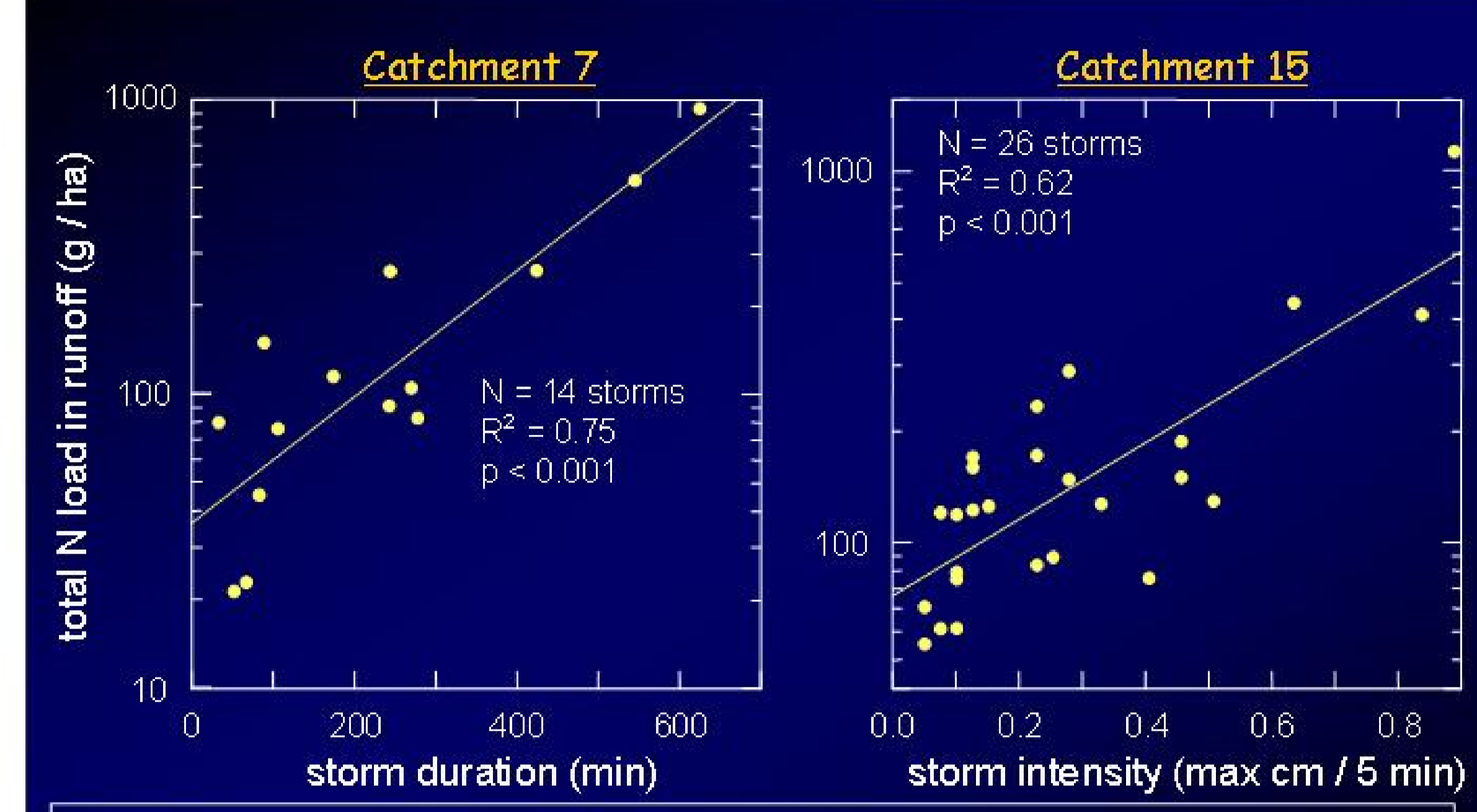
Figure 5. Storm attributes influence the load of total nitrogen exported from catchments in storm runoff. Different storm attributes, however, are related to N load in different catchments.
