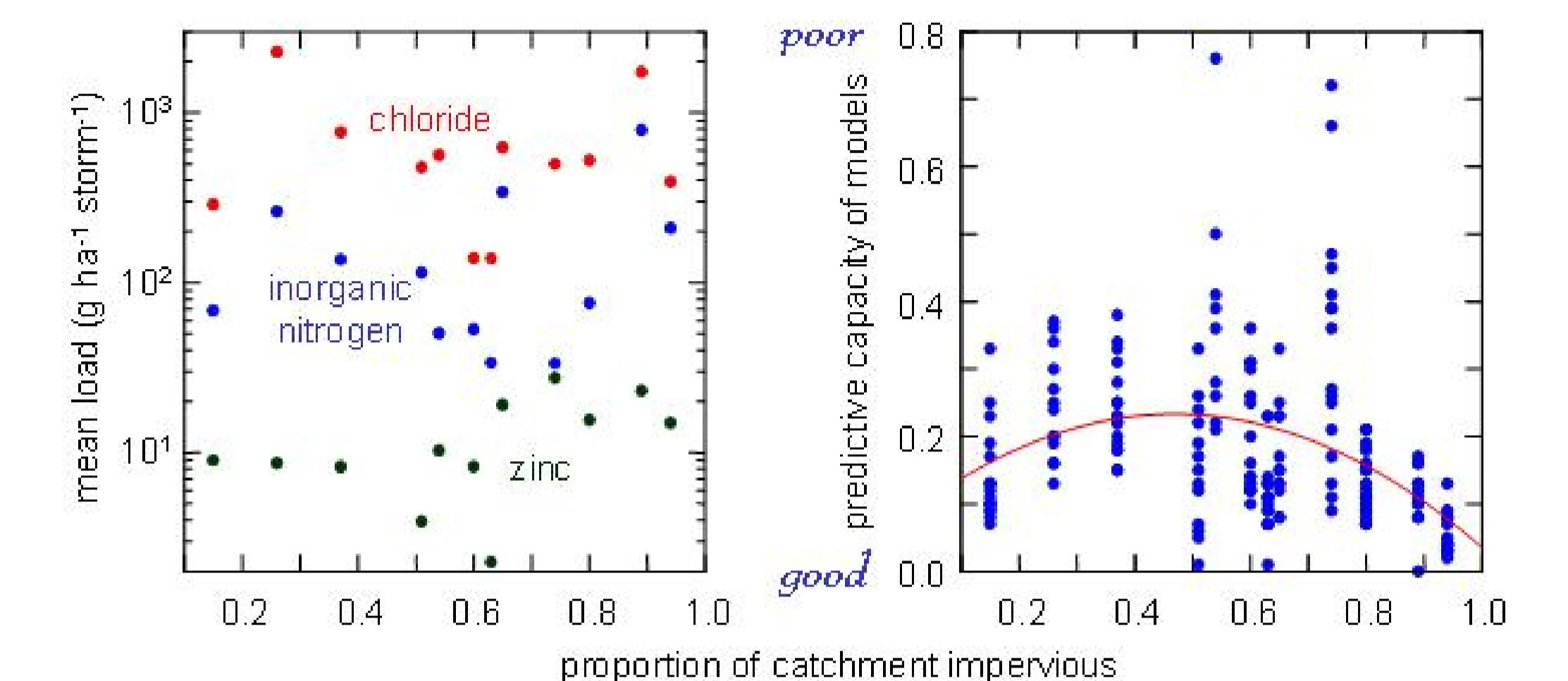
Figure 8. (Left) Mean (across all storm events) load of three different material species exported from a catchment plotted against proportion of impervious cover in the catchment. (Right) Y-axis value is the mean-square error in regression models that fit load as a function of storm attributes; each point is one such model fit to the load of a single material exported from a single catchment. X-axis value is the proportion of impervious cover in the catchments from which load was measured. Red line depicts a 2 nd -order polynomial (both terms p < 0.001).
