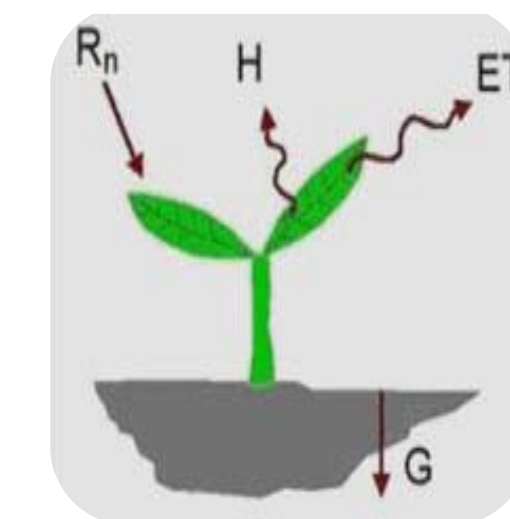
Figure 4: Energy balance fluxes
