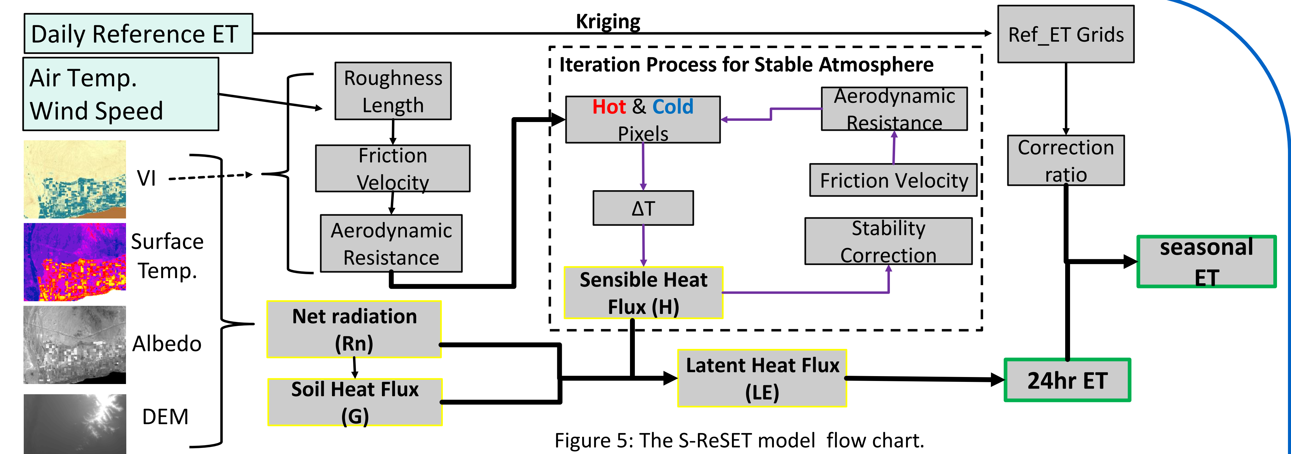
Figure 5: The S-ReSET model flow chart.
