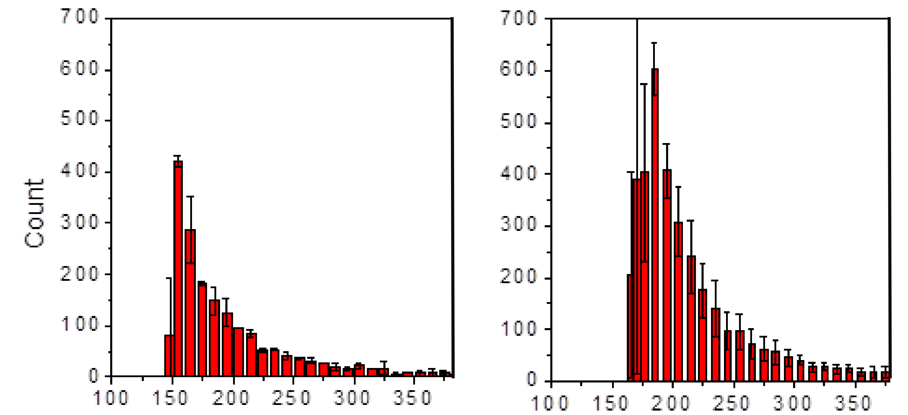
Spikes of titanium in the Salt River as they pass through the plasma of an ICP-MS.
