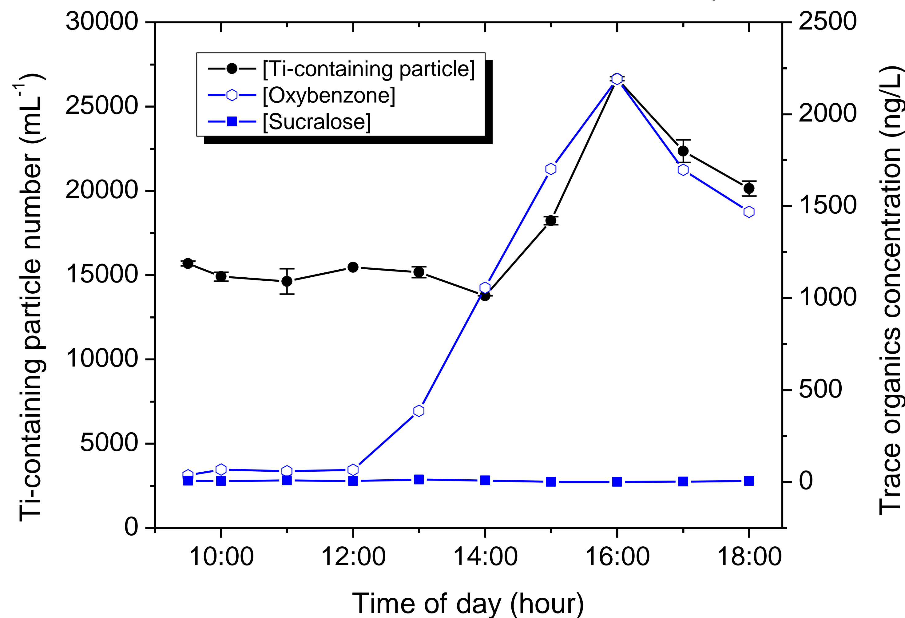
Concentrations of sunscreens and sucralose (wastewater) in the Salt River downstream of "Tubers" during a single day in summer.
