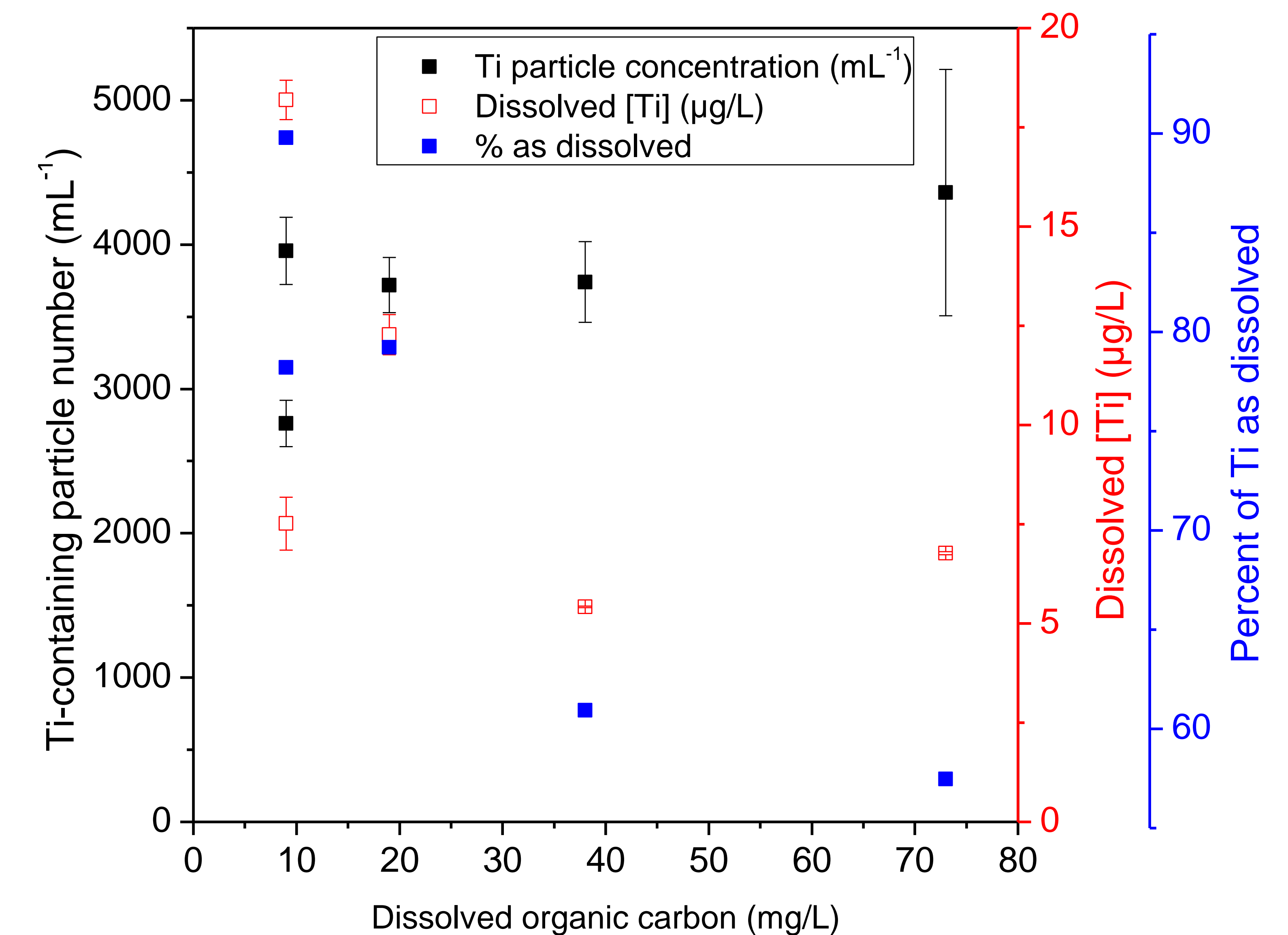
Measured titanium and dissolved organic carbon in swimming pools in Tempe.
