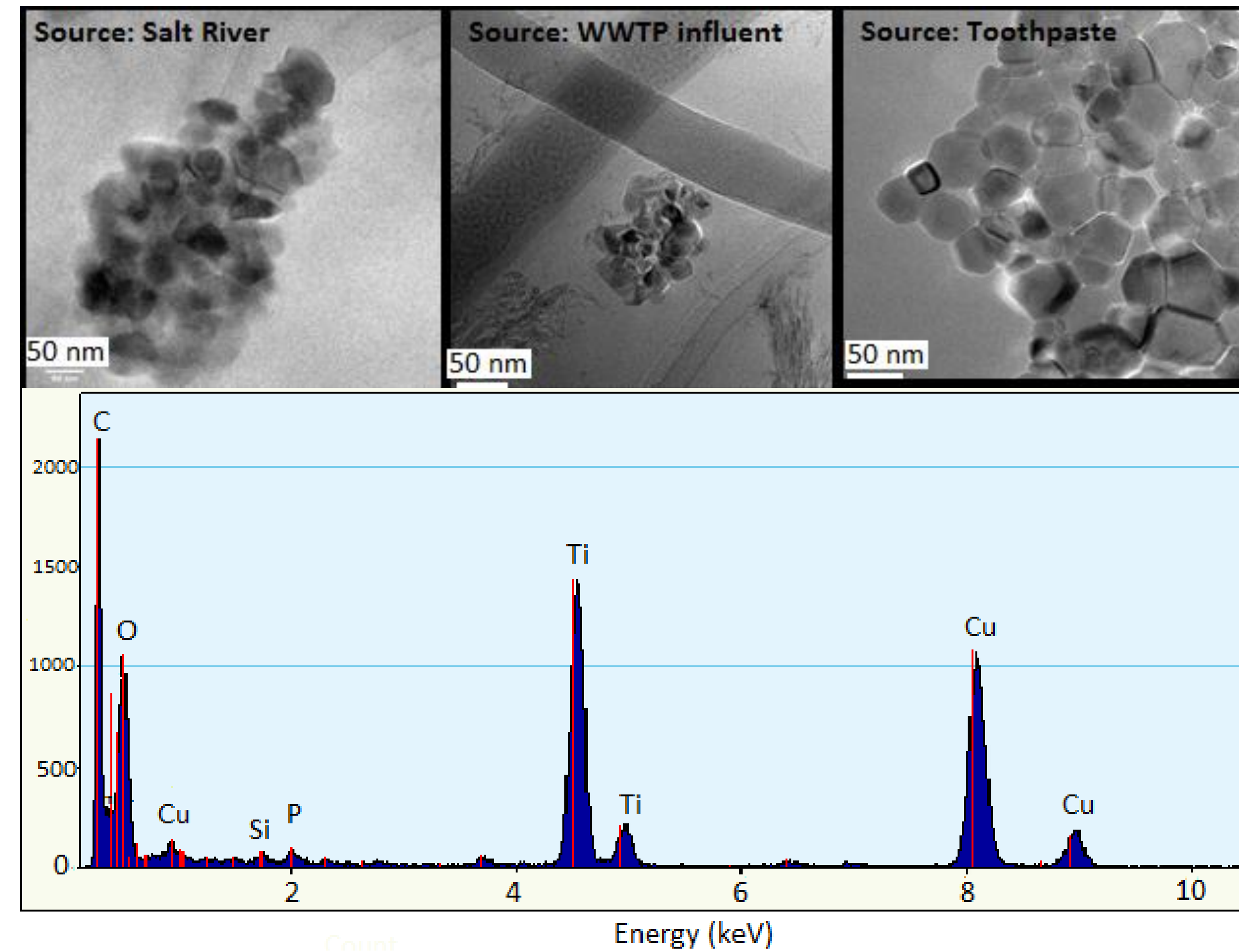
Identification of titanium containing nano particles in the Salt River, Mesa WWTP influent, and toothpaste.
