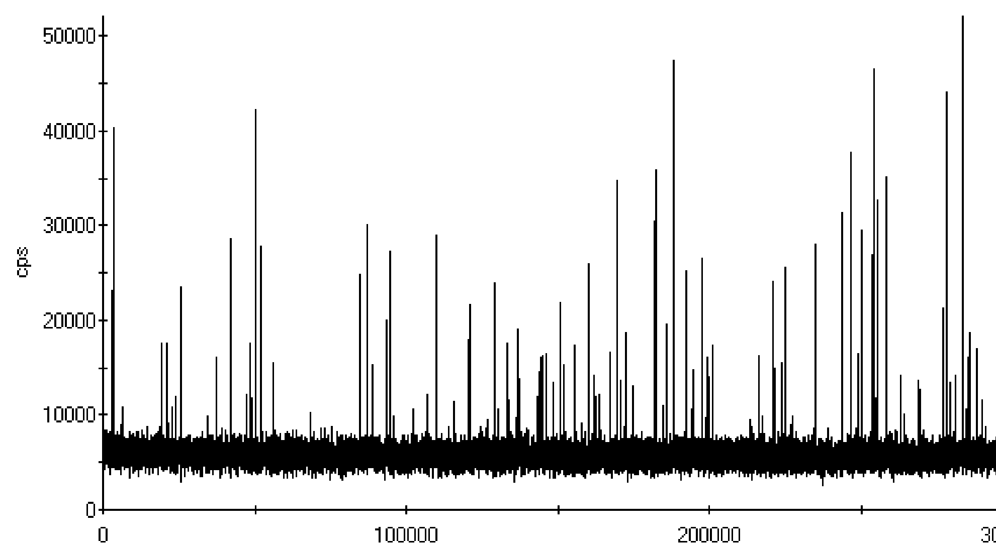
Example of raw single particle ICP-MS data of titanium spikes in a pool sample
