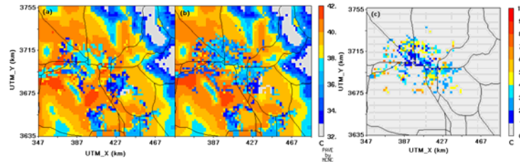
Figure 2: Simulated ground temperature using (a) USGS land use data and (b) 1998 satellite data, (c) differences between the two simulations.
