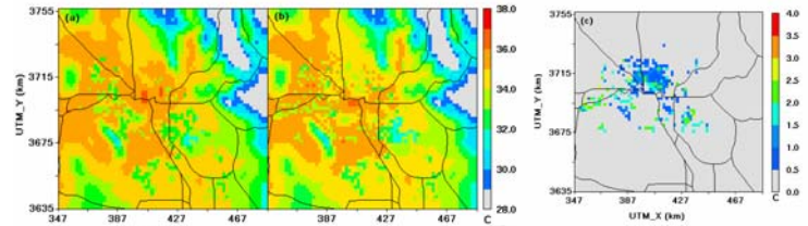
Figure 4: Simulated air temperature at 2m using (a) USGS land use data and (b) 1998 satellite data and (c) differences between the two simulations.
