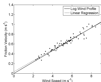
Friction velocity and wind speed measurements under near-neutral conditions at the Lost Dutchman State Park (LDP) site. The log-wind profile was used to predict z_0 = 0.27 m and u_* = 0.12 for the Sonoran desert sites.
