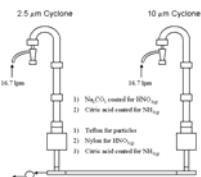
Schematic diagram of the denuder and filter sampler.
