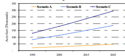
This graph illustrates the magnitude of difference of outdoor water use based on three separate scenarios of landscape irrigation. Scenario A assumes that by 2025 all housing units adopt xeriscapic landscapes; Scenario B assumes a partial conversion, and Scenario C assumes a continuation of turf dominated landscapes. In Scenario A the residents save as much as 76% of outdoor water, whereas those from Scenarios B and C save only 45% and 13% respectively.
