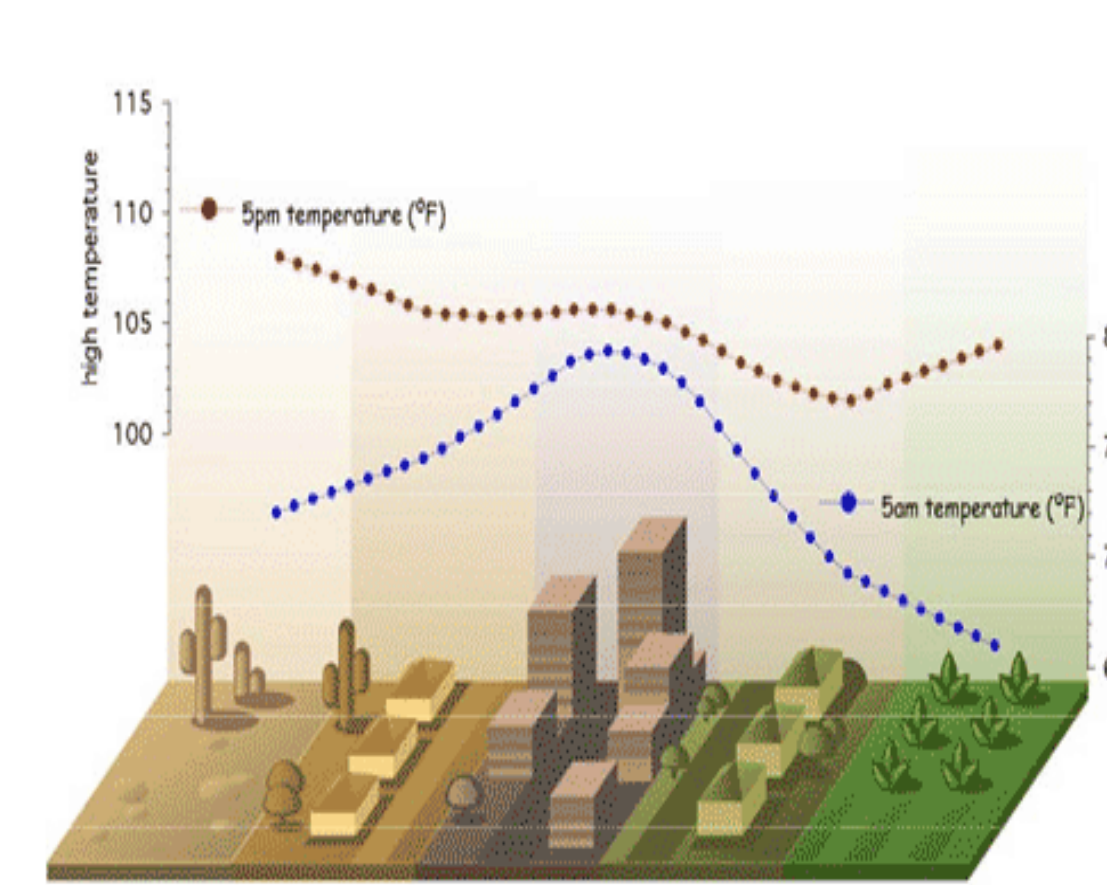
Figure 1: A diagram of the UHI at 5am and 5pm
