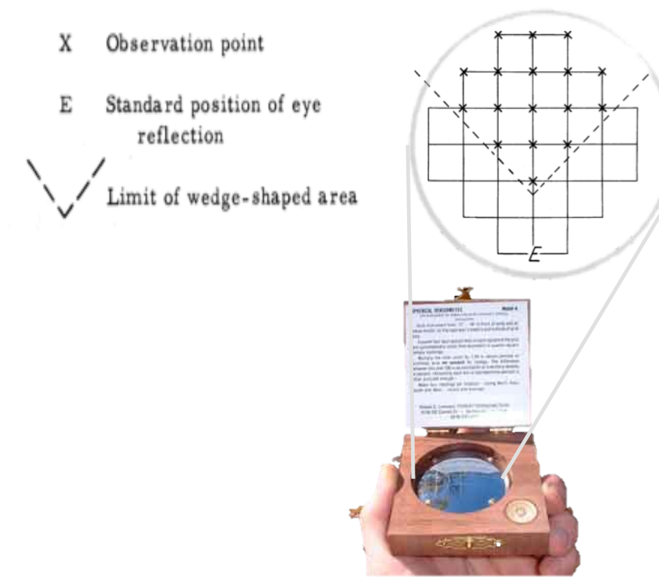
Figure 4: Densiometer with Strickler modifications.
