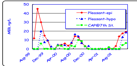
Figure 1. By releasing water from the hypolimnion, rather than the epilimnion, and occasionally using Colorado River water directly (bypassing L. Pleasant), MIB levels in the CAP Canal were consistently kept < 10 ng/L.
