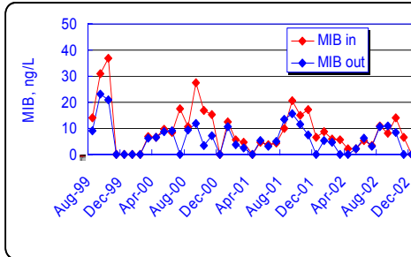
Figure 2. Effectiveness of PAC treatment at Val Vista WTP. MIB concentrations in treated water (MIB out) were generally lower than inlet concentrations, due to the use of PAC to adsorb MIB. Levels of PAC used was based upon MIB levels measured the previous week, communicated via the T&O Newsletter.
