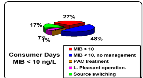
Figure 4. What worked? First, MIB concentrations would have been > 10 ng/L about half the time in 2001 without any management. Source switching (to avoid high MIB water at Deer Valley) and modification of Lake Pleasant releases were the most effective management practices, adding about 25% more consumer days with MIB < 10 ng/L. Finally, MIB was greater than 10 ng/L about 27% of the time.
