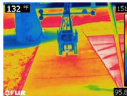
Figure 8: Infrared and visible images taken in Tempe, July 5, 2019, displaying surface temperatures as low as 96°F and up to 151°F. Surface temperatures were also taken with a handheld IRT.
